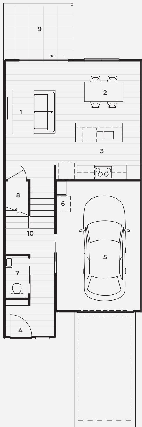
GROUND FLOOR
